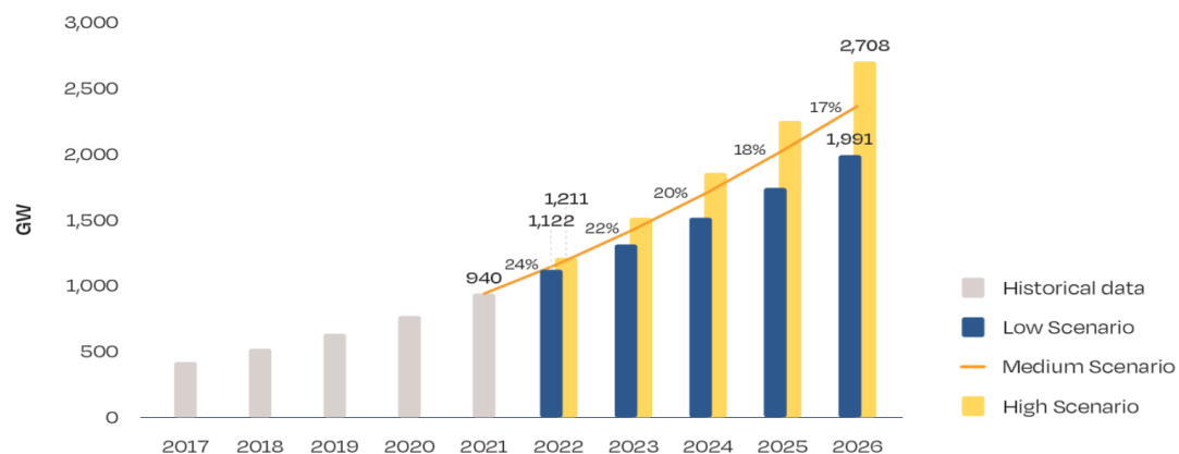
FIGURE 16 GLOBAL TOTAL SOLAR PV MARKET SCENARIOS 2022 - 2026
